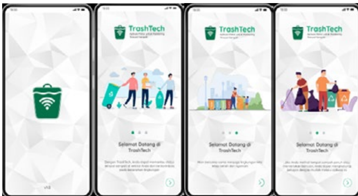
Figure 4. Splash Screen
