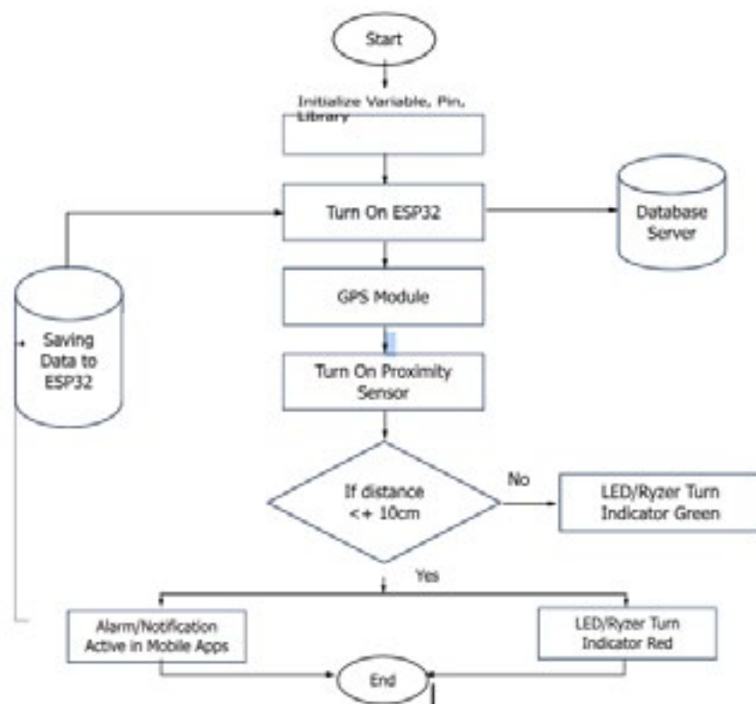
Figure 3. Flowchart System
